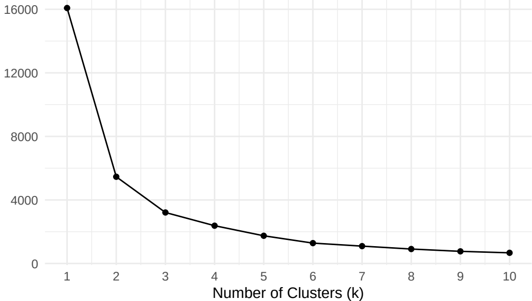
Elbow Method Graph Using Total WCSS
